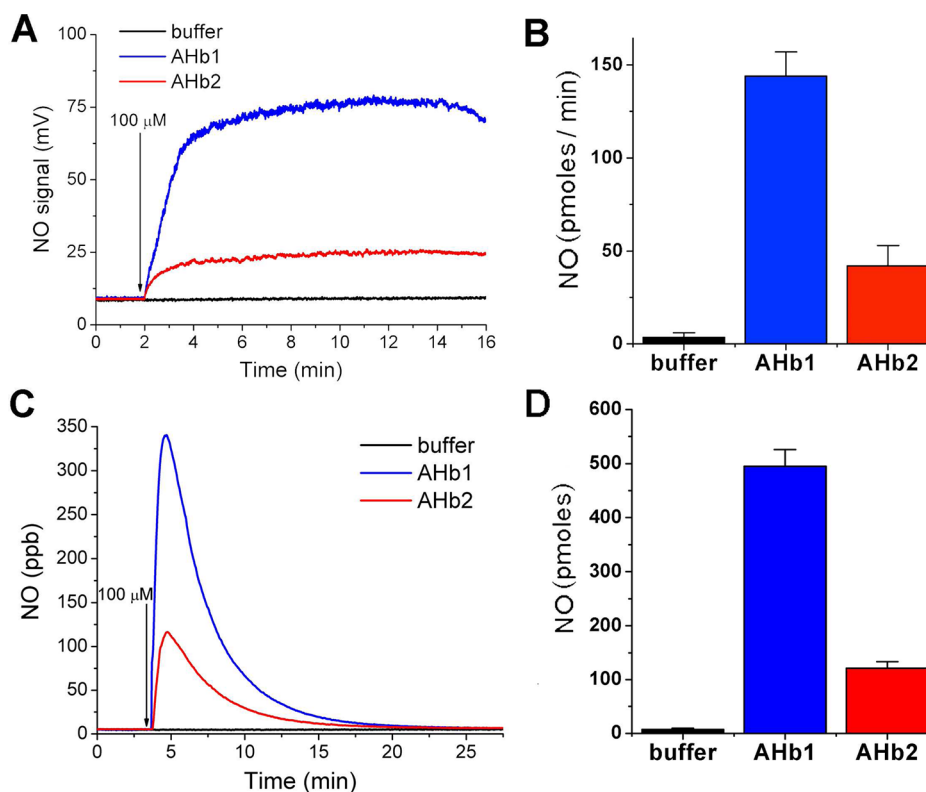
Figure 3. Reduction of nitrite by deoxy-AHb1 and -AHb2 generates NO gas during anoxia and hypoxia (2% oxygen). Chemiluminescence detection of NO gas emission during the anaerobic (A) and hypoxic (2% \text{O}_2 ) (C) reaction of nitrite with buffer alone (black), 25 \mu\text{M} deoxy-AHb1 (blue), or 25 \mu\text{M} deoxy-AHb2 (red). Arrows indicate the addition of nitrite in the specified amounts. Traces are representative of three or more separate experiments. (B and D) Quantification of the amount of NO detected for the reaction with 100 \mu\text{M} nitrite.
